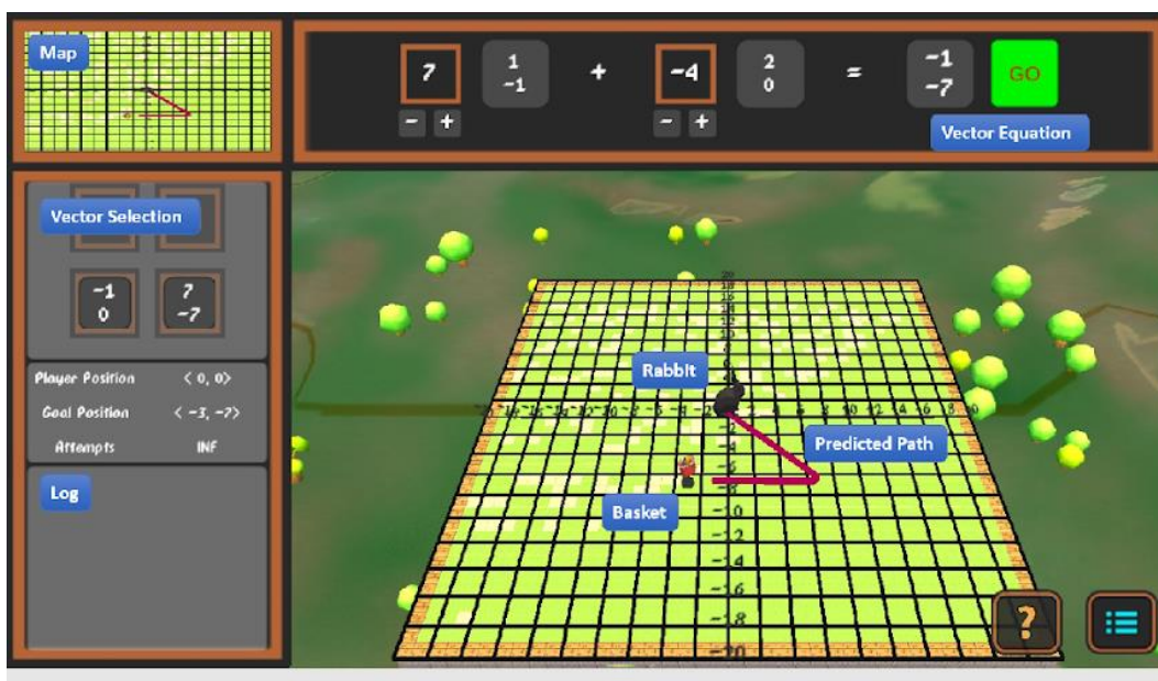
Figure 1. Sample Screen
